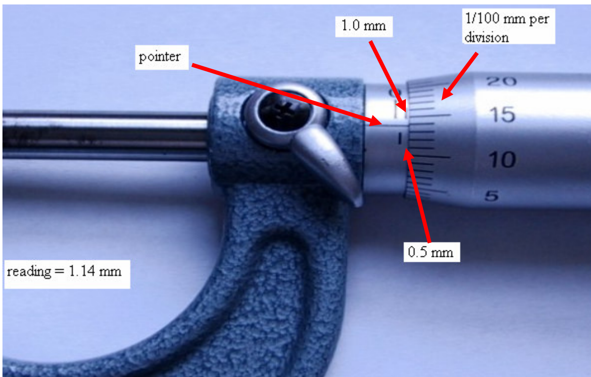
Micrometer screw gauge
