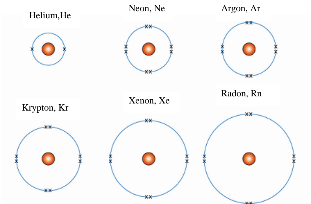
Electron arrangement in outer most shells in noble gases
